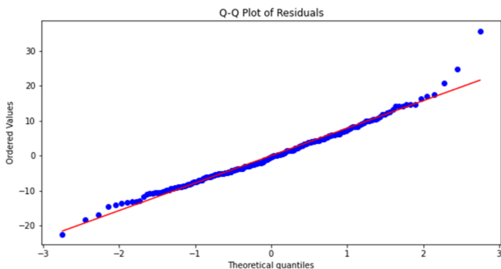
Figure 4.3.5: Q-Q Plot of Residuals
