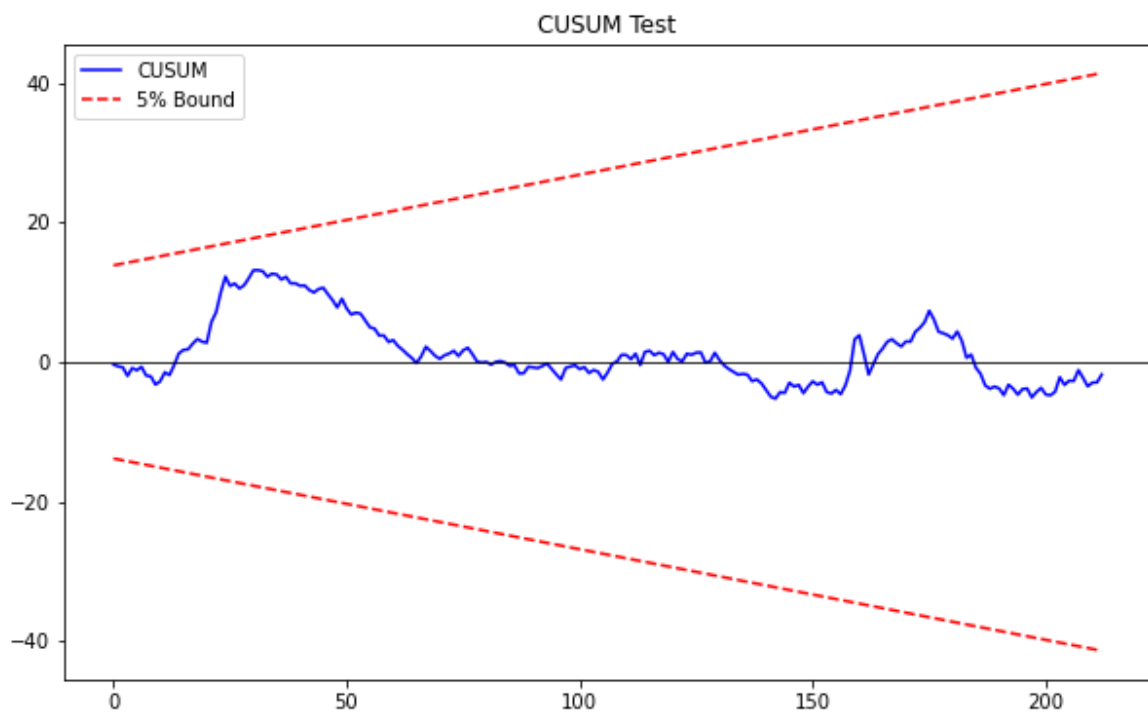
Figure 4.3: CUSUM Plot
