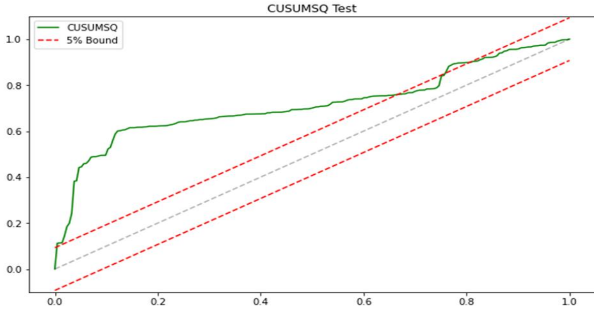
Figure 4.4: CUSUMSQ Plot
